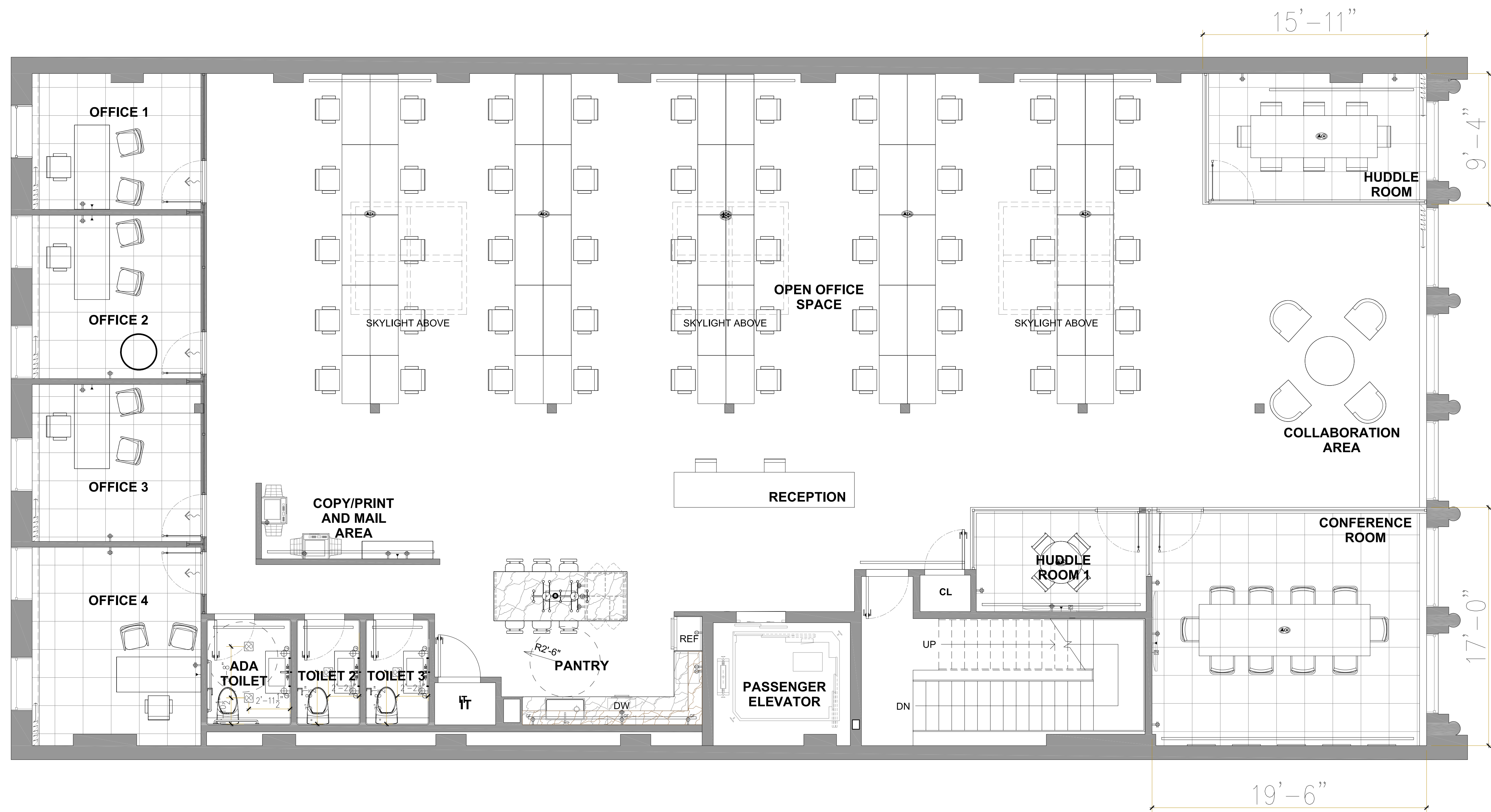
1 TYP. FLOOR PLAN SCALE: 1/4"=1'-0"
